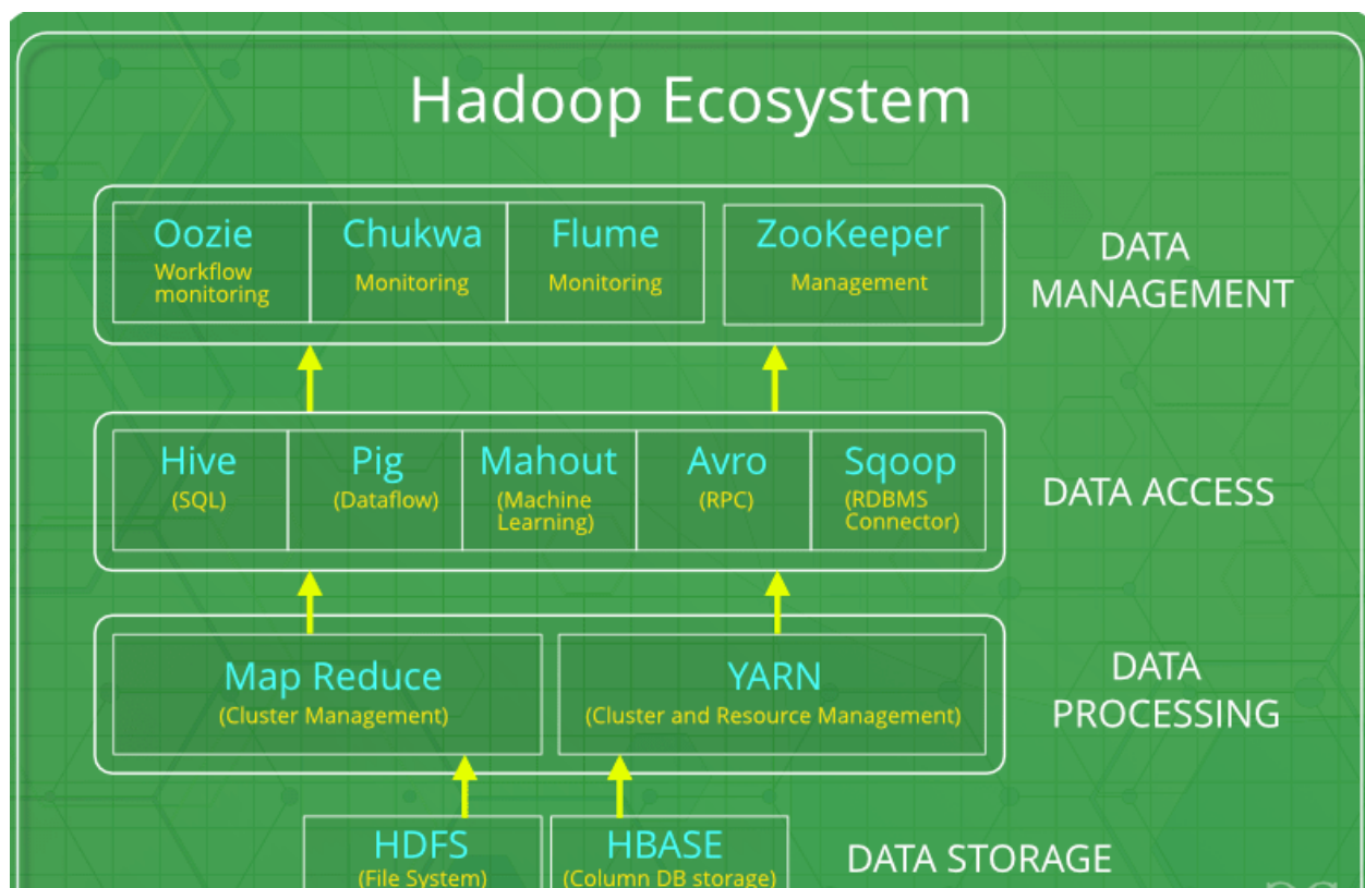
Figure 2.5 Hadoop Ecosystem
