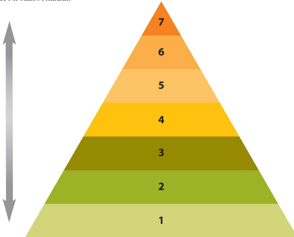
Figure 14.3 Maslow's Hierarchy
