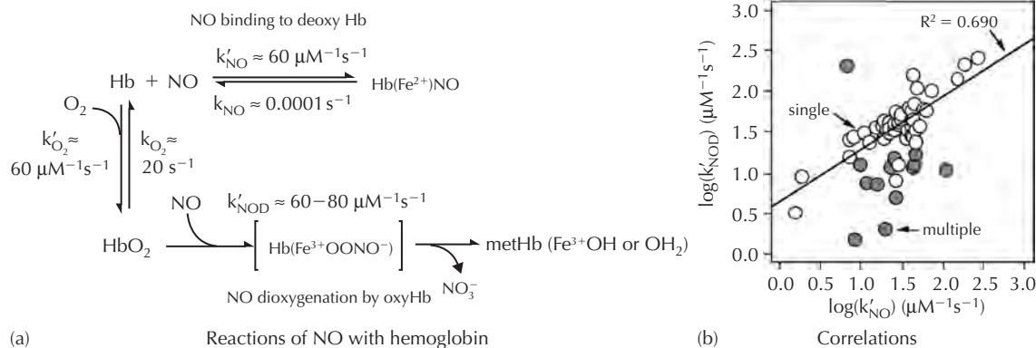
Figure 31.4 (a) Physiologically relevant reactions of NO with hemoglobin (Olson et al. , 2004).
