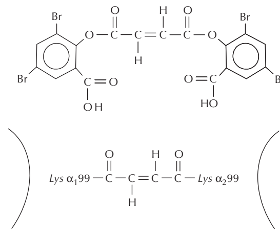
Figure 30.4 Structures of bis(3,5-dibromosalicyl) fumarate (DBBF) and the \alpha\alpha -hemoglobin crosslink (150).
