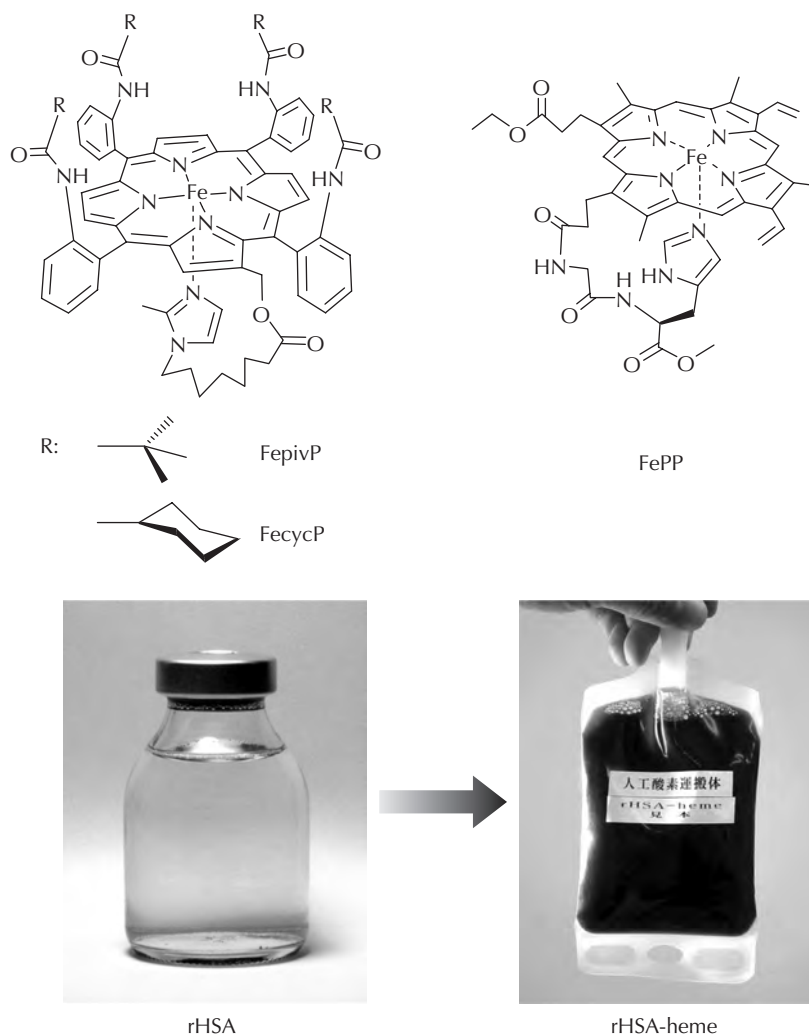
Figure 46.1 Super-structured heme derivatives for the albumin-heme hybrids and the red-colored rHSA-heme solution ([rHSA] = 5 g/dl). See color plate 23.
