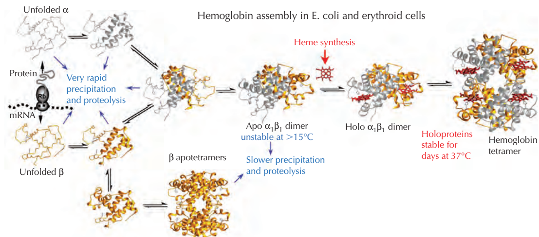
Plate 12 Scheme for hemoglobin assembly in both E. coli and erythroid cells. The thin lines represent unfolded regions and the large ribbons represent folded helices in the \alpha (silver) and \beta (gold) subunits. See Fig. 31.8.
