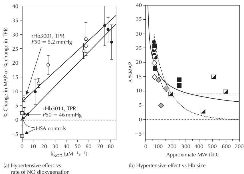
Figure 31.5 (a) Dependence of the hypertensive effect on the bimolecular rate of NO dioxygenation ( k'_{\text{NOD}} ) measured in vitro . Symbols: open circles, %MAP changes for three rHbs with allosteric mutations to vary P50 and three rHbs with distal pocket mutations to reduce NO scavenging (Table 31.1; Doherty et al. , 1998); closed circles, %TPR changes for three rHbs with allosteric mutations to vary P50 and two rHbs with multiple distal pocket mutations to reduce NO scavenging and increase P50 (Table 31.1 and Doyle et al. , 2001). (b) Dependence of the hypertensive effect on Hb size (molecular weight, see Olson et al. , 2004 for more details). Symbols: open diamonds, simple crosslinked Hbs (Rohlf et al. , 1998); closed circles, \Delta\% MAP changes in 10 per cent top-load experiments in rats for rHb tetramers with allosteric mutations (Doherty et al. , 1998); closed diamonds, \Delta\% MAP for Hbs decorated with PEG, POE, or o -poly-raffinose (Rohlf et al. , 1998); closed squares, \Delta\% MAP for various glutaraldehyde treated rHbs (Doyle et al. , 1999); half-filled squares, \Delta\% MAP changes for simple crosslinked Hb (XLHb), polyethylene glycol (PEG)-conjugated Hb, hydroxyethylstarch-conjugated XLHb, polymerized XLHb, and PEG-modified Hb vesicles (Sakai et al. , 2000). The solid, gray dotted, and black dashed lines represent fits to the following functions, respectively: a power law, a single exponential, and a single exponential with an offset.
