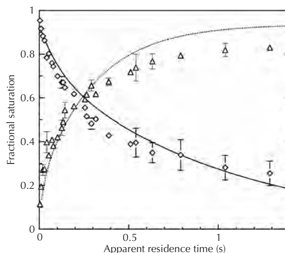
Figure 6.4 Comparison of experimental and model results for RBC/PolyBvHb 1 : 1 mixtures. Experimental data (10.2 g/dl total, pH 7.4) are plotted for uptake (triangles) and 50% oxygen gas equilibration release (diamonds). Humidified air was used to suffuse the capillary in the uptake experiments. For the release experiments, samples were equilibrated with humidified gas containing 50% oxygen. The corresponding theoretical simulations from the mathematical model described in this work are plotted as a dotted curve for uptake and as a solid curve for 50 per cent oxygen equilibration release. Shear augmentation is included in the simulations.
