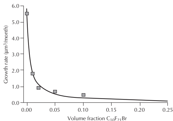
Figure 24.10 Droplet growth in an F -octyl bromide emulsion can be effectively repressed by adding a small amount of F -decyl bromide (from Weers et al. , 1994).
