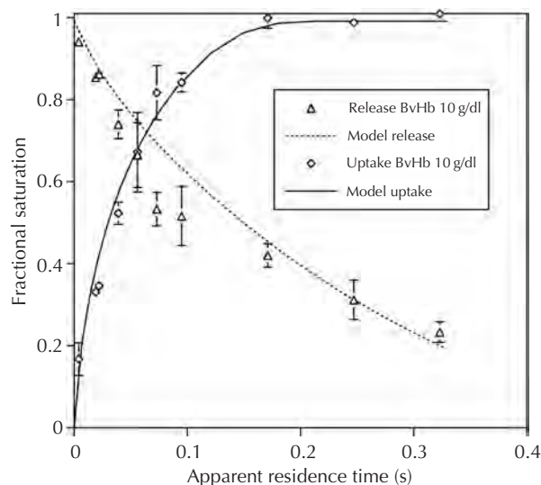
Figure 6.6 Hemoglobin solution oxygen uptake and release experiments for a 10- \mu\text{m} diameter capillary. Experimental determinations of hemoglobin oxygen saturation are presented as a function of residence time in the capillary. The data points represent measurements at five axial positions at two different flow rates. The error bars denote the standard deviation for replicate experiments. The curves are from predictive theoretical calculations. The good agreement between the experimental and theoretical values serves as a validation of the experimental apparatus.
