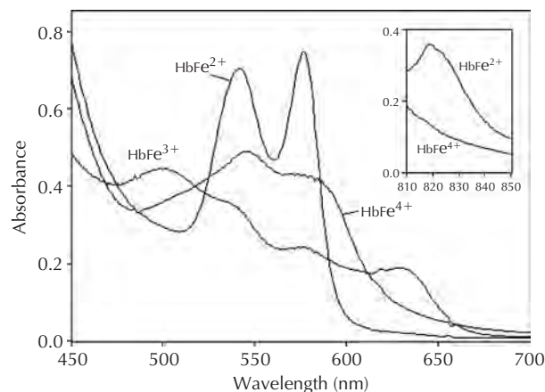
Figure 18.1 Optical spectra of hemoglobin oxidation products after reaction with hydrogen peroxide. Optical spectra of diaspirin cross-linked Hb ( \alpha\alpha -Hb) ( 50\ \mu\text{M} ) in phosphate buffer, pH 7.4, before the addition of \text{H}_2\text{O}_2 ( \text{HbFe}^{2+} ). The optical spectra of metHb ( 50\ \mu\text{M} ) before ( \text{HbFe}^{3+} ) and 2 minutes after the addition of 100\text{-}\mu\text{M} \text{H}_2\text{O}_2 ( \text{HbFe}^{4+} ). Peaks, which appear at 545 and 585 nm respectively, represent the characteristic profile of the intermediate, ferryl redox state. The addition of \text{H}_2\text{O}_2 to ferrous hemoglobin generates an identical spectrum to the ferryl spectrum. The production of ferryl Hb can be confirmed by addition of 2-mM sulfide, which can generate sulfHb ( \text{HbSFe}^{2+} ) from the ferryl, indicated by the peak at 620 nm (see insert).
