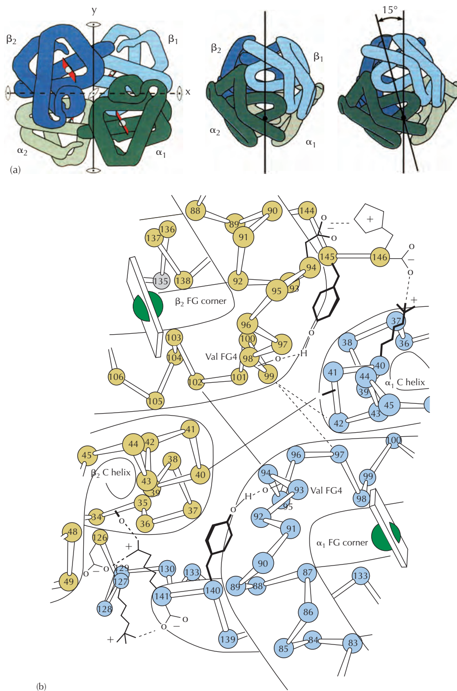
Plate 4 The allosteric transition in HbA. (a) Overview of the allosteric transition (reproduced with permission from Eaton et al. , 1999). The allosteric transition consists mainly of a sliding and a rotating motion of the \alpha_1\beta_1 dimer with respect to the \alpha_2\beta_2 , with a consequent rearrangement of the \alpha_1\beta_2 interface and the symmetric \alpha_2\beta_1 . (b) Details of the amino acid contacts at the \alpha_1\beta_2 interface (modified after Dickerson and Geis, 1983). See Fig. 29.2.
