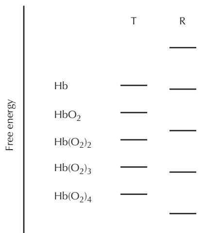
Figure 29.4 Free energy diagram of the two-state allosteric model of Monod et al. (1965). The ligand binding free energy of ^T\text{Hb} is smaller than that of ^R\text{Hb} , but ^T\text{Hb} is favored by (RT \ln L_0) ; hence in the absence of oxygen ^T\text{Hb} is prevalent; however, each successive molecule of oxygen that binds favors ^R\text{Hb} , until this allosteric state becomes prevalent (usually between the second and the third molecules of oxygen).
