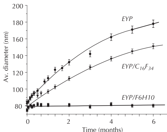
Figure 24.12 Fluorocarbon-hydrocarbon diblock molecules can stabilize fluorocarbon emulsions very effectively. Stabilization with diblock C_6F_{13}C_{10}H_{21} (F6H10) is more effective than with a heavy PFC of similar molecular weight, C_{16}F_{34} , which only reduces the solubility of the dispersed PFC phase but not the interfacial tension (from Krafft et al. , 2004). Note the preservation of very small particle sizes over time when the diblock is used.
