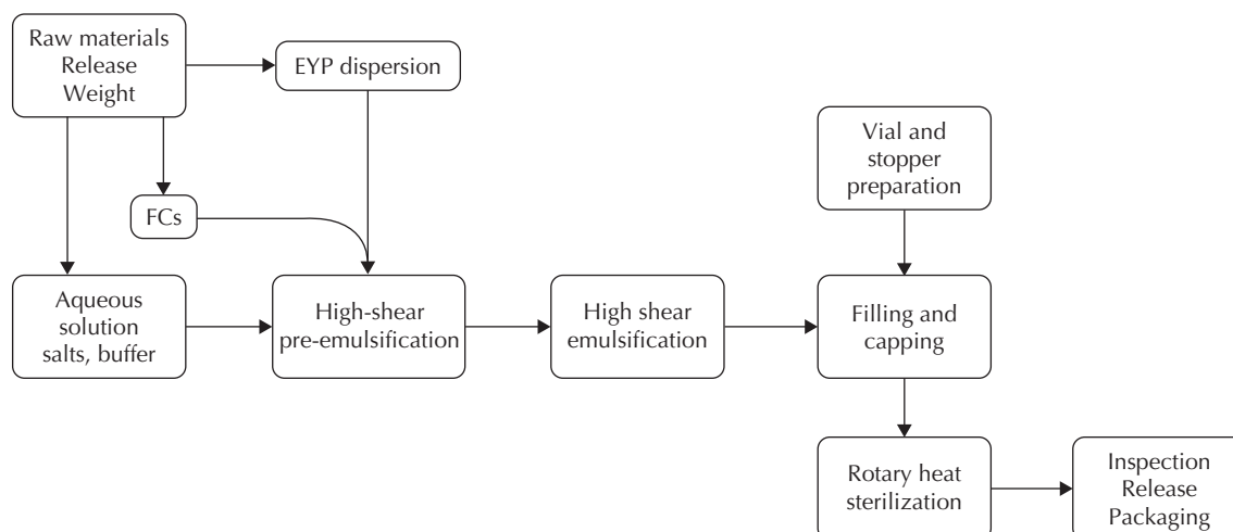
Figure 24.8 Schematic fluorocarbon emulsion production flowchart.
