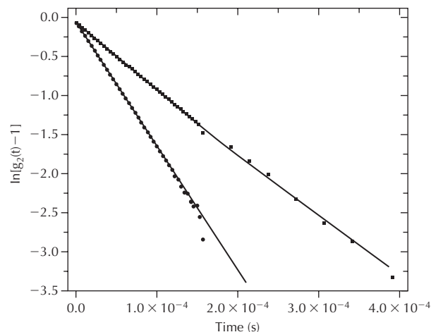
Figure 32.2 Autocorrelation function of HbA (circles) and Hb Prisca (squares) transformed according to the cumulant analysis method. The solid lines are a second-order polynomial fit of the transformed data. The different slopes reflect the different sizes of the two samples. In both cases, the linearity of the slopes indicates the presence of a homogeneous population of molecules (Fronticelli et al. , 2001).
