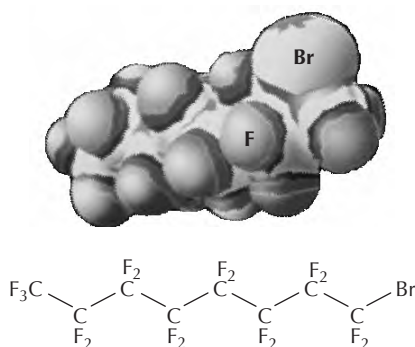
Figure 24.5 Molecular model of F -octyl bromide, showing the lipophilic bromine atom protruding at the end of the linear chain.
