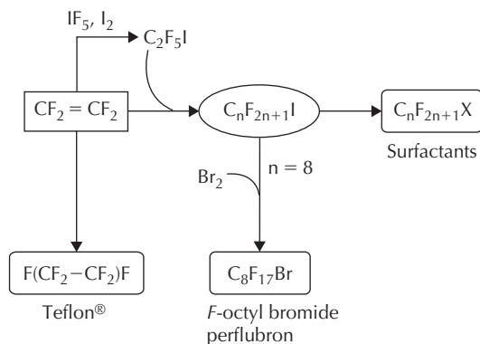
Figure 24.6 Industrial process for F -octyl bromide (perflubron) synthesis: one step from a pivotal perfluorochemical, F -octyl iodide.
