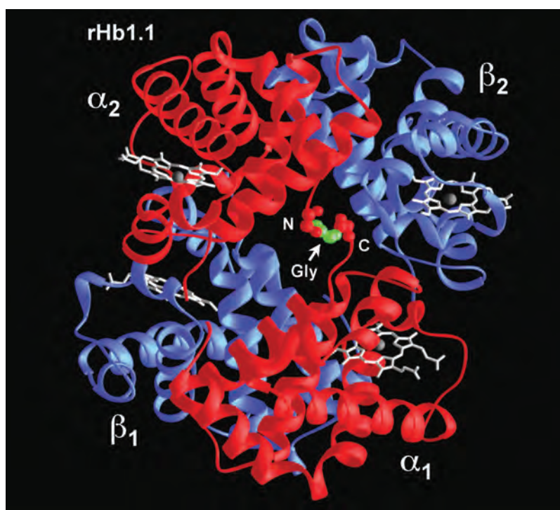
Plate 7 Structure of deoxy rHb1.1 showing the single glycine linker between the C-terminus of \alpha_1 and the N terminus of \alpha_2 (PDB accession code 1C7C (Brucker, 2000). See Fig. 31.1.
