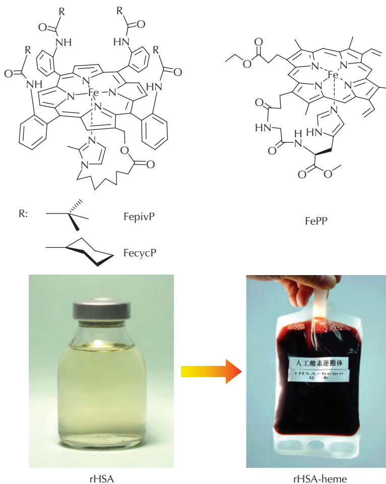
Plate 23 Super-structured heme derivatives for the albumin-heme hybrids and the red-colored rHSA-heme solution ([rHSA] = 5 g/dl). See Fig 46.1.
