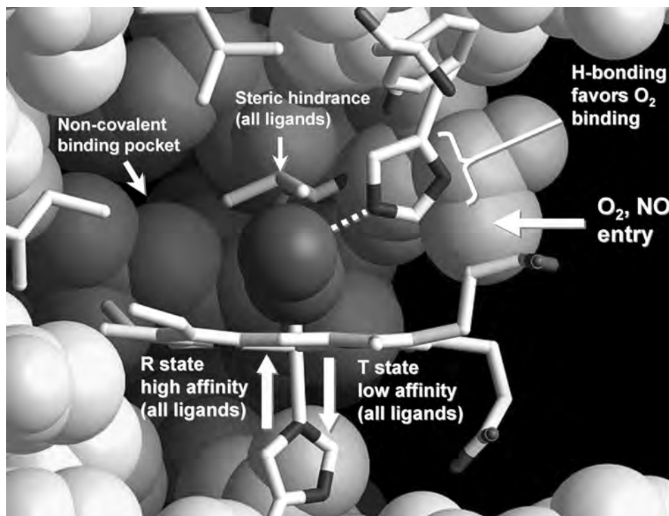
Figure 31.2 The structure of the active site of recombinant sperm whale MbO 2 (Quillin et al. , 1993). The amino acid side chains and their helical positions are, starting with the proximal histidine underneath the heme and rotating clockwise: HisF8, Ile(Mb) or Leu(Hb)G8, LeuB10, ValE11, PheCD4, and HisE7, the distal histidine. The non-covalent binding site is where all ligands are captured before bond formation and where they reside before exiting the protein during dissociation. It is also the location for the capture of NO during the dioxygenation reaction. The factors governing O 2 affinity are labeled in white and taken from Olson and Phillips (1996, 1997) and Dou et al. (2002). See color plate 8.
