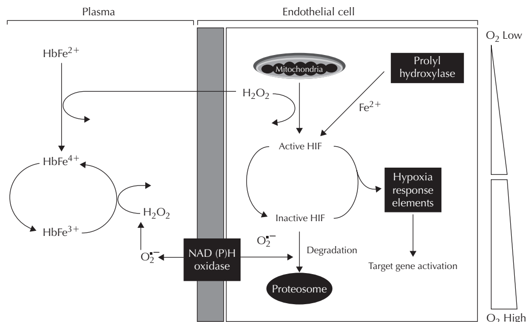
Figure 18.3 Proposed roles for HBOCs in the modulation of cell-signaling pathways. Both ROS and RNS can regulate transcription and translation processes. NADPH oxidase converts O_2 to superoxide ( O_2^{\bullet -} ) under normoxia, inactivating HIF-1 \alpha and targeting it for proteosomal degradation, thus acting as an oxygen sensor. The mitochondrial cytochrome oxidase system represents a second potential O_2 sensor. Decreased O_2 increases O_2^{\bullet -}/H_2O_2 and stabilizes HIF-1 \alpha . The cytoplasmic prolyl hydroxylase represents a third potential O_2 -sensing mechanism by which decreased O_2 availability prevents hydroxylation of specific HIF-1 \alpha proline residues; the opposite occurs during normoxia. Introduction of hypoxia (low oxygen) and HbFe^{+2} leads to changes in both hemoglobin redox states and redox-sensitive cell-signaling pathways. Hemoglobin competes with endogenous reactions that consume peroxides, resulting in increased HIF-1 \alpha expression. The reaction of hemoglobin with H_2O_2 leads to series of transitions between the ferrous ( HbFe^{2+} ), ferric ( HbFe^{3+} ) and ferryl ( HbFe^{4+} ) redox states.
