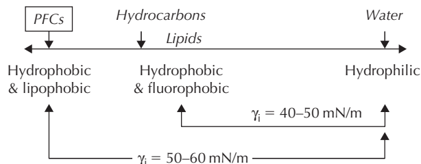
Figure 24.1 The relative positions of fluorocarbons, hydrocarbons and water on a polarity scale: fluorocarbons are more hydrophobic than olive oil, and are oleophobic as well.
