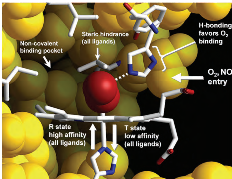
Plate 8 The structure of the active site of recombinant sperm whale MbO 2 (Quillin et al. , 1993). The amino acid side chains and their helical positions, starting with the proximal histidine underneath the heme and rotating clockwise: HisF8, Ile(Mb) or Leu(Hb)G8, LeuB10, ValE11, PheCD4, and HisE7, the distal histidine. The non-covalent binding site is where all ligands are captured before bond formation and where they reside before exiting the protein during dissociation. It is also the location for the capture of NO during the dioxygenation reaction. The factors governing O 2 affinity are labeled in white and taken from Olson and Phillips (1996, 1997) and Dou et al. (2002). See Fig. 31.2.
