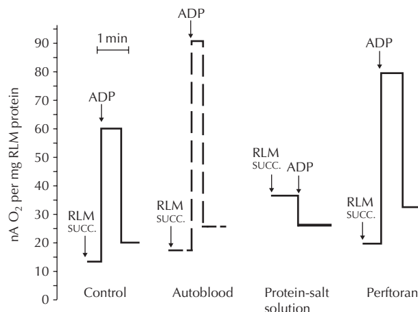
Figure 26.2 Diagrams of polarographic registration of respiratory rate of rat liver mitochondria (RLM) during oxidation of 5 mM potassium succinate (succ.) and phosphorylation of 150 \mu M ADP. Each curve is a mean value of six measurements (s.e.m. < 10\% of mean value). RLM were isolated in 6 h after blood replacement by scavenged autologous blood, protein-salt solution or by Perftoran (Hb content decreased from 16.0 \pm 1.4 to 5.0 \pm 0.6 g/dl in both groups). Incubation medium for RLM: 250 mM sucrose, 10 mM KCl, 10 mM Tris-HCl (pH 7.4), 3 mM KH_2PO_4 , 3 mM MgCl_2 , (RLM protein 2–3 mg/ml), t 26°C. After blood replacement by protein-salt solution or by Perftoran, animals were kept at PO_2 of 550–600 mmHg. (Based on data from Maevsky et al. , 1999.)
