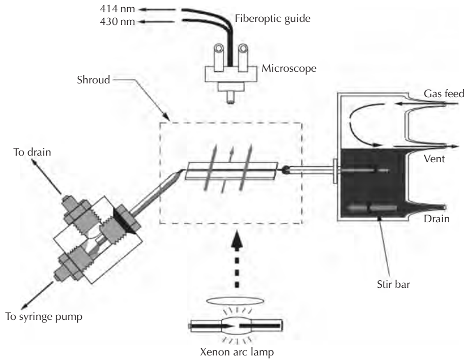
Figure 6.3 Schematic of experimental apparatus for artificial capillary – the microflow system and microspectrophotometric systems.
