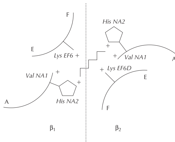
Figure 30.1 Reaction of diphosphoglycerate (2,3-DPG) and deoxyhemoglobin. The molecule fits into the central cavity of hemoglobin and forms salt bridges with valine NA1(1) \beta , histidines NA2(2) \beta , H121(143) \beta and lysine EF6(82) \beta . A, E, and F refer to specific hemoglobin helices and NA is the sequence from the amino-terminals to the A helix.
